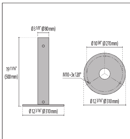
Mounting Base
